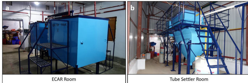
Fig. 2. Digital photographs of the 10,000 LPD capacity pilot plant at Dhapdhapi High School. a) ECAR Room: Contains the two ECAR reactors in which electrolysis occurs b) Tube Settler Room: Contains the tube settler, flocculation chamber, and subsequent tertiary treatment systems for particle separation.
