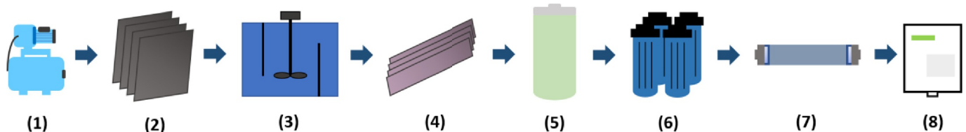
Fig. 3. Schematic representation of the treatment process at the Dhapdhapi pilot plant: 1) raw water pump, 2) ECAR reactors, 3) flocculation chamber, 4) tube settler, 5) rapid sand filter, 6) micron filters, 7) ultraviolet disinfection system, 8) automatic dispensing unit.
