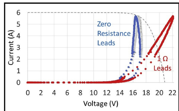
Fig. 11. The grey shadow is the diode curve from Fig. 9 with total resistance of 0.08 Ohms due to leads and a shunt resistor. The blue curve is the voltage if the leads to the diode had no resistance, and the red curve is if the leads had a resistance of 1 Ohm. (For interpretation of the references to colour in this figure legend, the reader is referred to the Web version of this article.)
