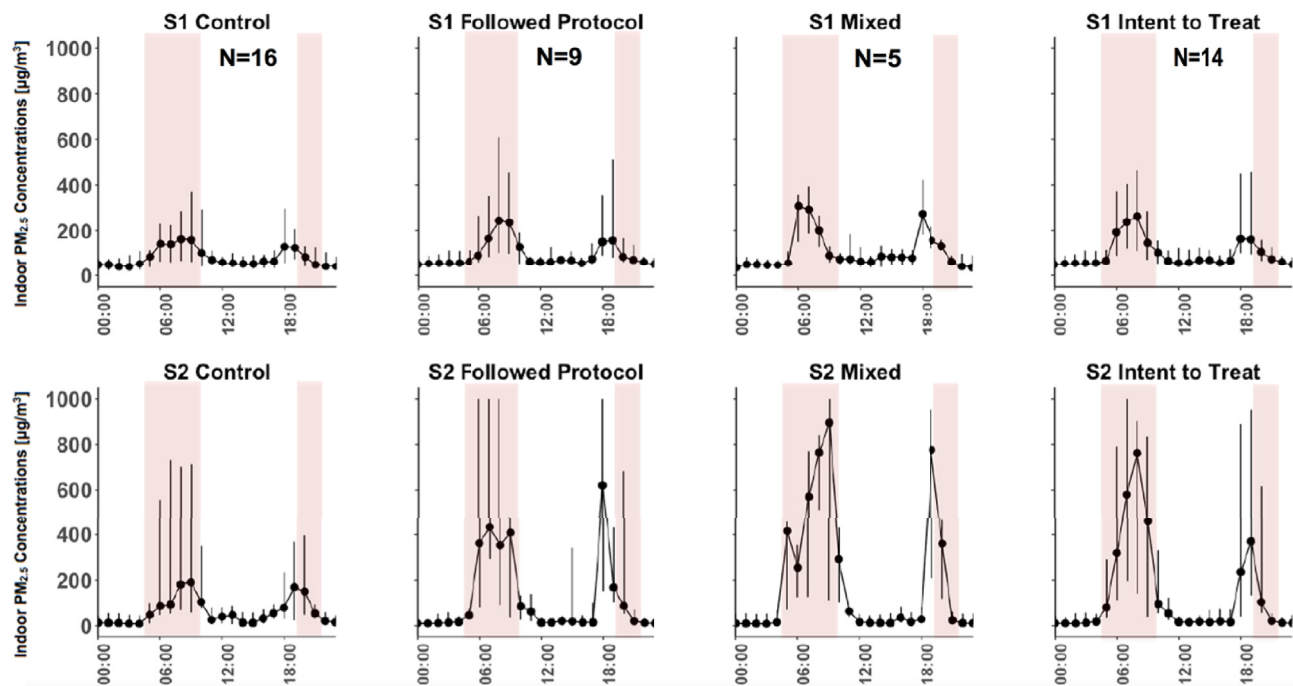
Fig. 2. Average hourly indoor PM_{2.5} concentrations by season and stove use category. Shaded regions indicate fixed-window cooking periods. Error bars represent the 25th and 75th quartiles. Sample size for each season and stove category are indicated at the top of each panel. “S1” (top row) is pre-intervention; “S2” (bottom row) is post-intervention.
