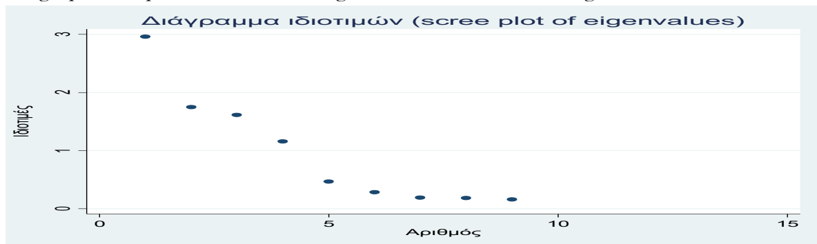
Figure 2. Eigenvalue chart
