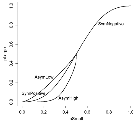
FIGURE 1 QRE selection in the experimental Stag Hunt games. p_{Small} (p_{Large}) = probability of contributing by small (large) player in the almost symmetric games SymPositive with \left(\frac{c_i}{G_i}\right) = \left(\frac{4}{10}, \frac{4}{10}, \frac{8}{20}, \frac{8}{20}\right) and k = 4 and SymNegative with \left(\frac{c_i}{G_i}\right) = \left(\frac{-4}{-10}, \frac{-4}{-10}, \frac{-8}{-20}, \frac{-8}{-20}\right) and k = 1 . p_{Small} (p_{Large}) = probability of lowest (highest) cost player in the asymmetric games AsymLow with \left(\frac{c_i}{G_i}\right) = \left(\frac{4.5}{20}, \frac{5}{20}, \frac{5.5}{20}, \frac{6}{20}\right) and AsymHigh with \left(\frac{c_i}{G_i}\right) = \left(\frac{2}{20}, \frac{4}{20}, \frac{6}{20}, \frac{8}{20}\right) and k = 4 in both cases. Remarks: All paths of QRE start at QRE(0) = (0.5, 0.5, 0.5, 0.5) and end at the Nash equilibrium QRE(1,096) = (0, 0, 0, 0) in the positive frame and QRE(1,096) = (1, 1, 1, 1) in the negative frame. In the almost symmetric games, the strategies of the two small and the two large players are equal. For the asymmetric games the strategies of the middle cost players are not indicated
