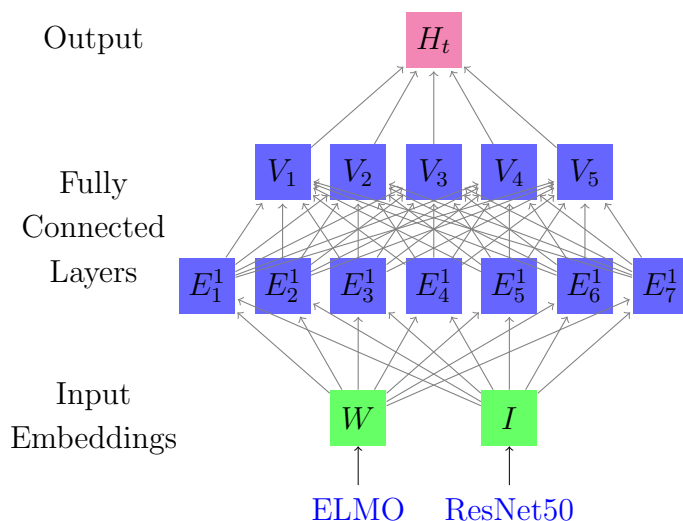
FIGURE 15. SingleTask + ELMO model. Product text is mapped to W and image is mapped to I of dimensions 256 and 2048. For illustration purpose, we only show two hidden layers with dimension 7 and 5 respectively. In practice, we use three layers with dimension 2048, 1024, and 256. The output is price for one time period t .
