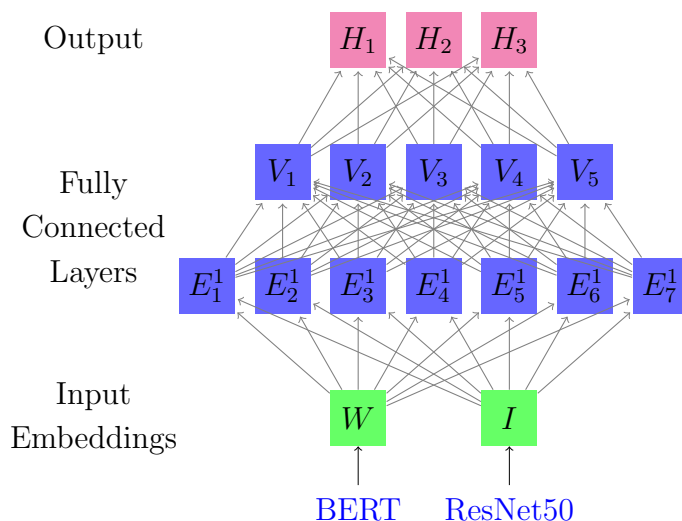
FIGURE 16. MultiTask + BERT. Product text is mapped to W and image is mapped to I of dimensions 3072 and 2048 respectively. For illustration purpose, we only show two hidden layers with dimension 7 and 5 respectively, and output is of dimension 3. In practice, we use three layers with dimension 2048, 1024, and 256, and the output is a price vector over T = 72 time periods.
