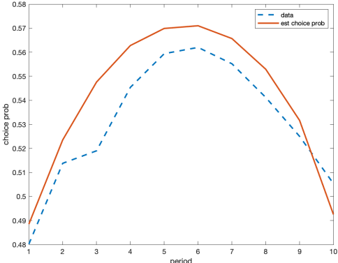
(c) DGP 3
