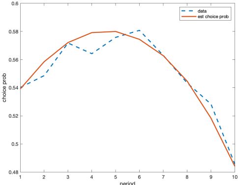
(a) DGP 1
