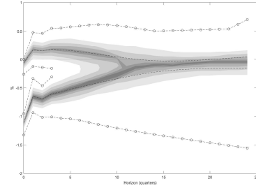
(b) Inflation to \varepsilon_t^{mp} : impulse response draws
