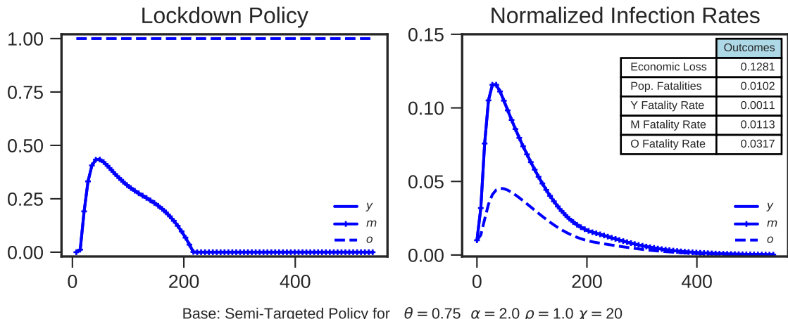
Figure 5: Optimal semi-targeted policies for baseline.
