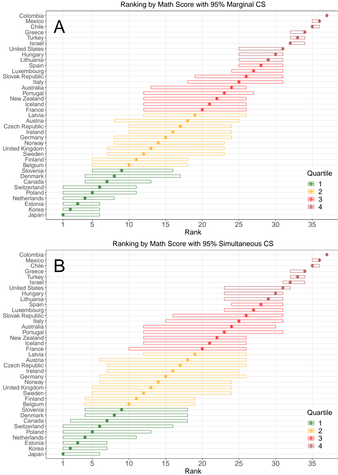
Figure 19: Panel A: for each OECD country, we plot its rank by math score and the 95% marginal confidence set ("CS"). Panel B: for each OECD country, we plot its rank by math score and the 95% simultaneous confidence set ("CS"). Different quartiles of the rankings are indicated with different colors.
