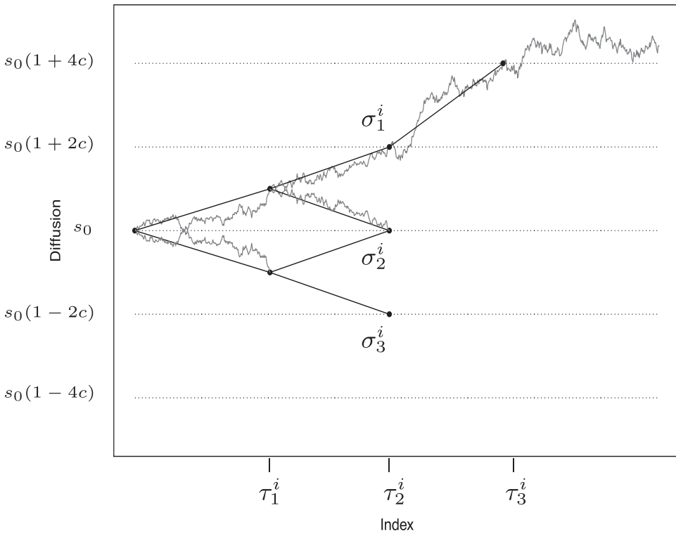
FIGURE 3 Illustration of the stopping times defined in (22), (23) resp. (24). The first stopping takes place when the process reaches either the first upper or lower boundary s_0^i(1 \pm c) . Starting from the upper boundary the next stopping takes place if the process increases to the level s_0^i(1 + 2c) , decreases to the level s_0^i(1 - 2c) or crosses the level s_0 . In case the process reached the upper level a third stopping occurs at \tau_3^i
