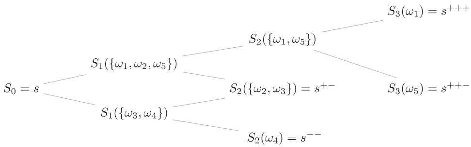
FIGURE 4 The embedded binomial model for the follow-the-trend strategy with positive drift. The filtration generated by the final states is generated by each \{\omega_i\} for i = 1, 4, 5 and \{\omega_2, \omega_3\} . We also denote the resulting outcomes by s = s_0, s^+, s^-, \dots and indicate this notation at some places
