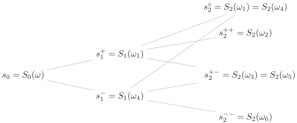
FIGURE 1 The considered trinomial model with T = 2 time steps. The first step is binomial, the second step is also (recombining) binomial with an additional top state \{\omega_1, \omega_4\}
