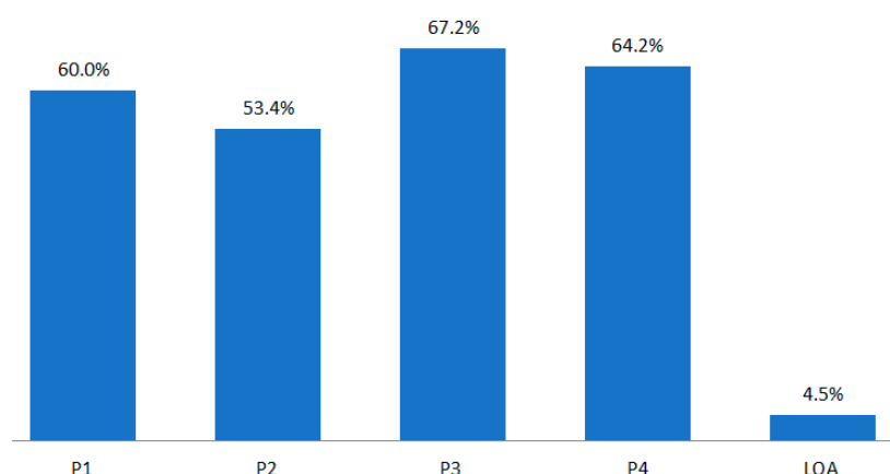
Figure 3. POS/LOA by BLA drug class for the whole period (1970–2017).
