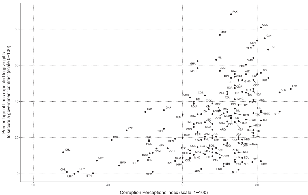
FIGURE 1 Comparison of the corruption values of the Enterprise Surveys and the corruption Perceptions Index Source: Transparency International (2018), World Bank (n.d.-b).
