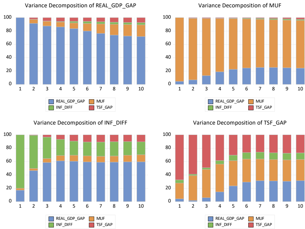
Figure 12: Variance Decomposition
