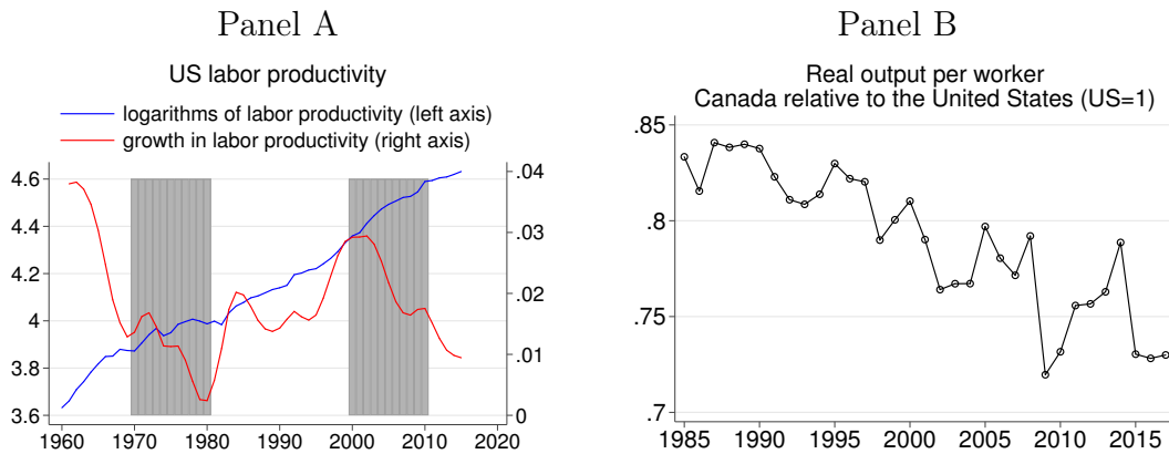
Figure 1: Aggregate productivity in the US and Canada
