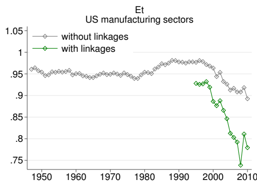
Figure 9: E_i in the US manufacturing sectors over time, year-by-year shares
