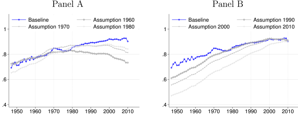
Figure A.2: E_i in the US, assuming undistorted factor shares in various years
