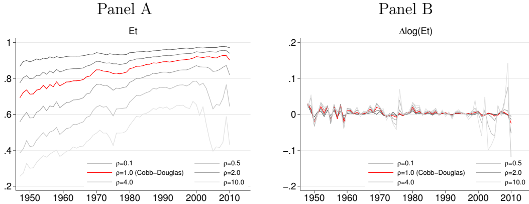
Figure 8: \mathbf{E}_t and \Delta \log(\mathbf{E}_t) , different \rho
