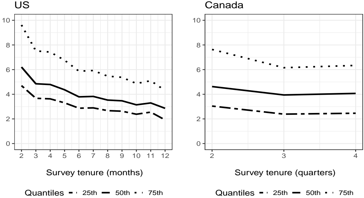
Figure 6: Estimated volatility
