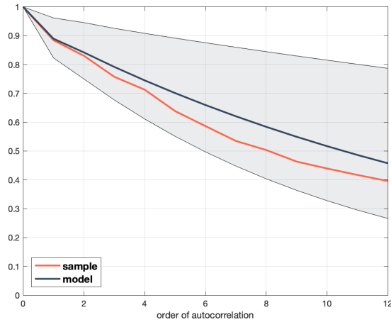
FIGURE 4. Autocorrelations of the statistical discrepancy. The solid indigo line contains the autocorrelations implied by model IP at point estimates. Shaded area is a pointwise 95% confidence interval for each lag.
