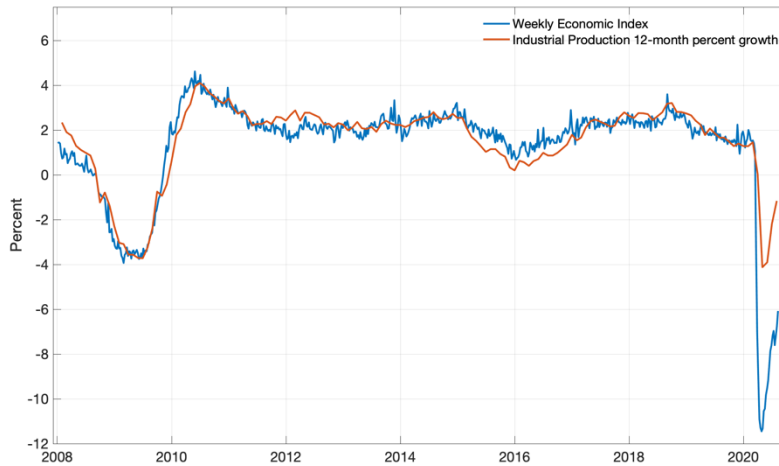
Figure 5: WEI and Industrial Production
