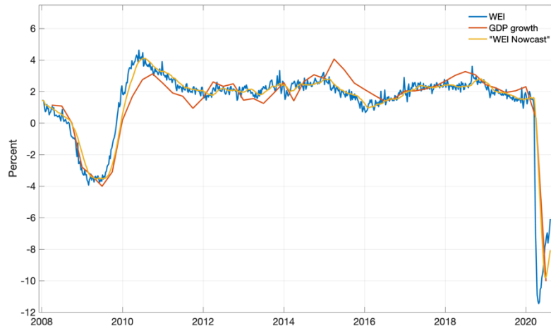
Figure 4: WEI and GDP growth
