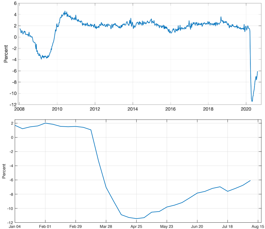
Figure 1: Weekly Economic Index (WEI)
