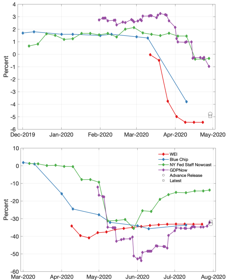
Figure 6: Progression of WEI and GDP nowcasts in 2020
