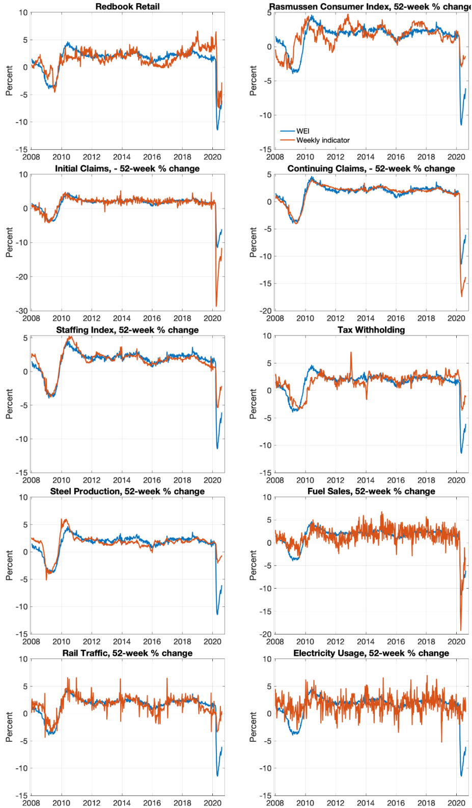
Figure 2: Weekly Variables and WEI
