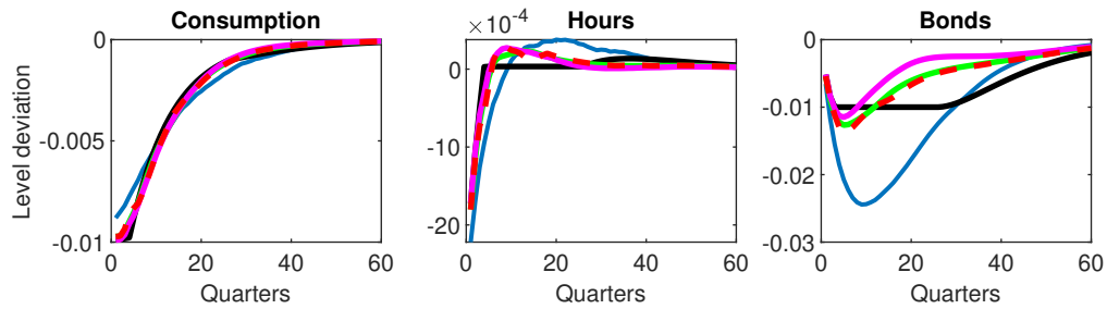
Chart 7: Comparison of impulse response to a technology shock in the borrowing constraints model using different solution methods
