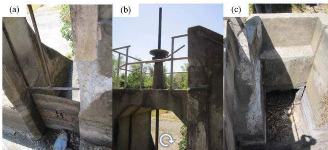
Figure 1A-95. (a) The wooden sluiceway gate; (b) the operating screw of the sluiceway gate; (c) the intake gate with broken regulator
