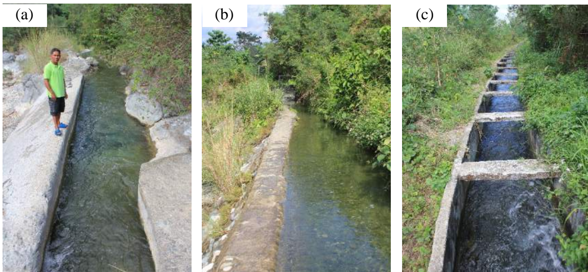
Figure 1A-39. (a) Intake channel at the side of the river just after the dam; (b) continuation of the intake channel; (c) the main canal just after the check gate Source: Author's capture
