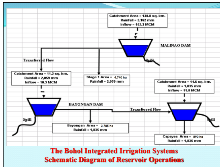
Figure 24. Schematics of the water transfer from Malinao down to Capayas reservoir.
