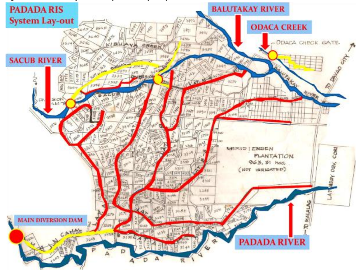
Figure 40. Canal layout and parcellary map of Padada RIS with other intake dams.
