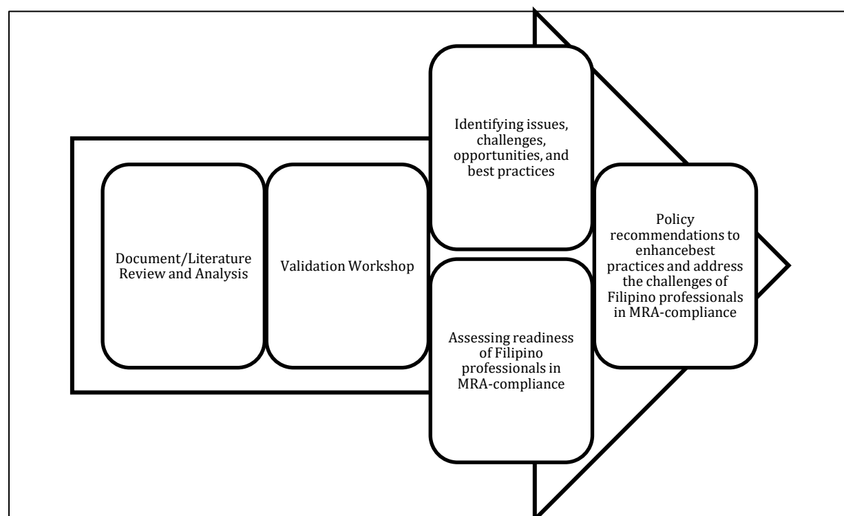
Figure 5. Methodological outcomes
