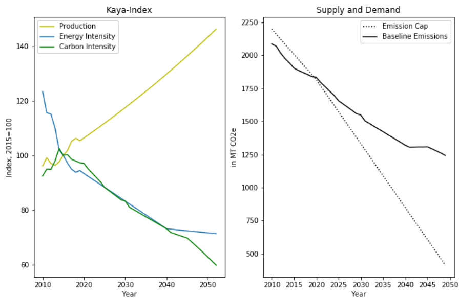
Figure 1: Kaya indices, baseline emissions and emission cap in the no-shock scenario
