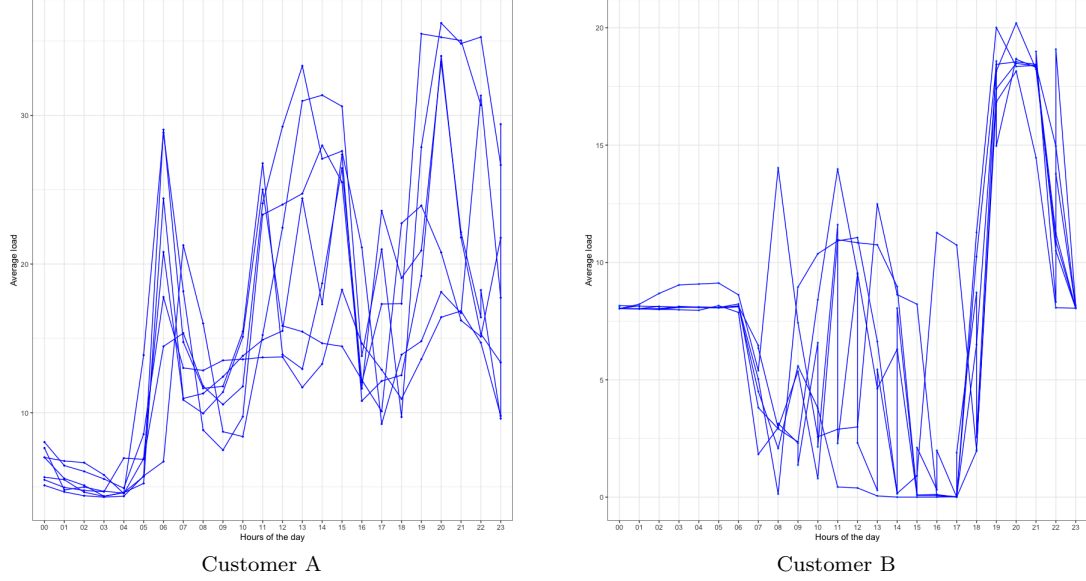
Figure 3. The figure shows the daily average load for a randomly sampled week for two randomly drawn customers. The unit of measurement is Watt.
