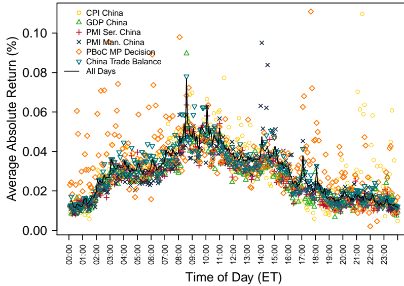
Figure 5: China macroeconomic announcement dates volatility. It shows the average absolute five-minute USD/MXN return over the sample period, January 14, 2008, through November 8, 2017, for dates where at least one following China’s macroeconomic announcements is released: the Consumer Price Index, the revisions to the Gross Domestic Product, manufacturing and services Caixin Purchasing Managers’ Indexes (PMI), Trade Balance and Monetary Policy decision by The PBoC, the times of these announcements variate from 20:00 ET to 6:00 ET. Sources: Own estimations with data from Bloomberg.
