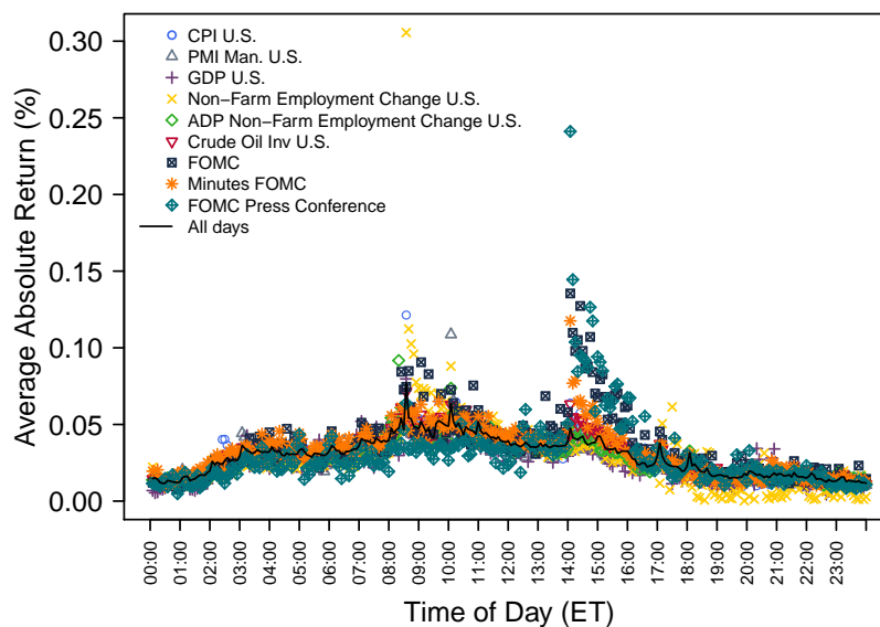
Figure 4: U.S. macroeconomic announcement dates volatility. It shows the average absolute five-minute USD/MXN return over the sample period, January 14, 2008, through November 8, 2017, for dates where at least one following U.S. macroeconomic announcements is released: the Consumer Price Index, the revisions to the Gross Domestic Product the Non-Farm Employment Change and its estimation (ADP) at 8:15; at 10:00 and 10:30 the Manufacturing PMI and Crude Oil Inventories respectively; at 9:00 and at 14:00 the monetary policy decisions by the FED, minutes and press conference from the FOMC. It can be observed that around the announcements' release time the volatility increases, the most noteworthy increments are linked to monetary policy announcements. Sources: Own estimations with data from Bloomberg.
