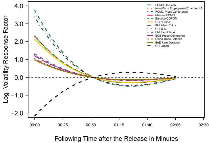
Figure 7: After announcement 2 hours effect. The figure shows the effects two hours after selected macroeconomic announcements for the five-minute USD/MXN absolute returns over the sample period, January 14, 2008 through November 8, 2017. Sources: Own estimations with data from Bloomberg and Banco de México’s website.
