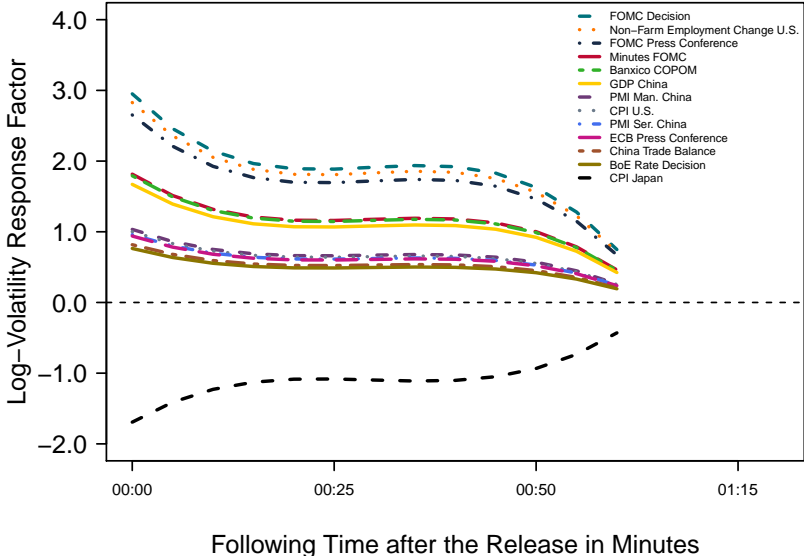
Figure 6: After announcement 1 hour effect. The figure shows the effects an hour after selected macroeconomic announcements for the five-minute USD/MXN absolute returns over the sample period, January 14, 2008 through November 8, 2017. Sources: Own estimations with data from Bloomberg and Banco de México’s website.
