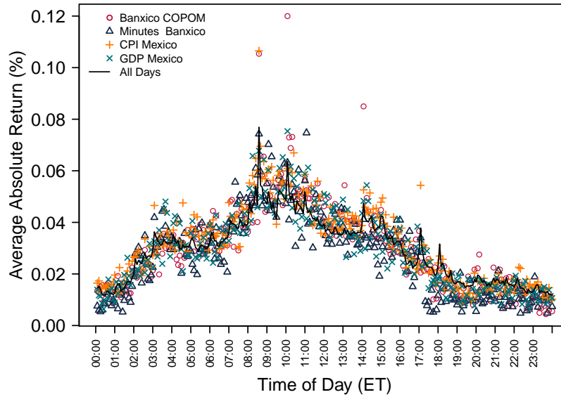
Figure 3: Mexico macroeconomic announcement dates volatility. It shows the average absolute five-minute USD/MXN return over the sample period, January 14, 2008, through November 8, 2017, for dates where at least one following Mexico’s macroeconomic announcements is released: the Consumer Price Index and the revisions to the Gross Domestic Product at 9:00; at 14:00 the monetary policy decisions and minutes of Banxico. Sources: Own estimations with data from Bloomberg and Banco de México’s website.
