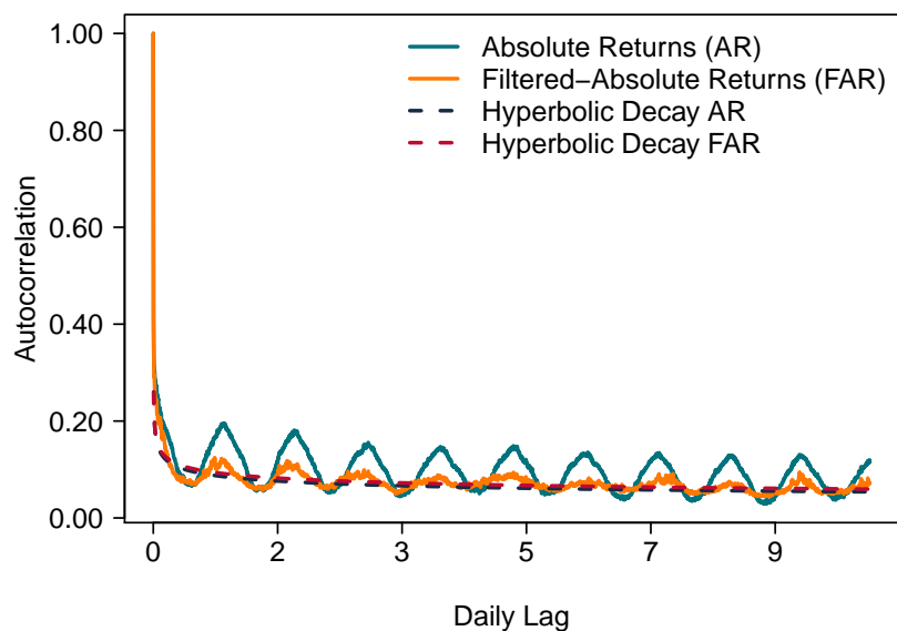
Figure 8: Absolute and filtered-absolute returns correlograms. It shows the autocorrelations for the five-minute USD/MXN absolute and filtered-absolute returns over the sample period, January 14, 2008, through November 8, 2017. The filtered returns are obtained by using the following equation \frac{|x_{t,n} - \mu|}{\hat{s}_{t,n}} . Sources: Own estimations with data from Bloomberg and Banco de México’s website.
