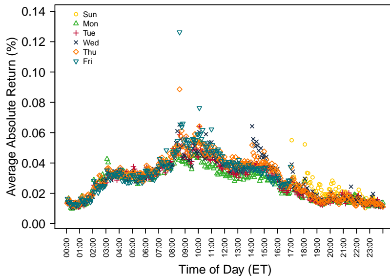
Figure 2: Day of the week. It shows the average absolute five-minute USD/MXN return over the sample period (January 14, 2008, through November 8, 2017) from Sunday to Friday. Sources: Own estimations with data from Bloomberg.
