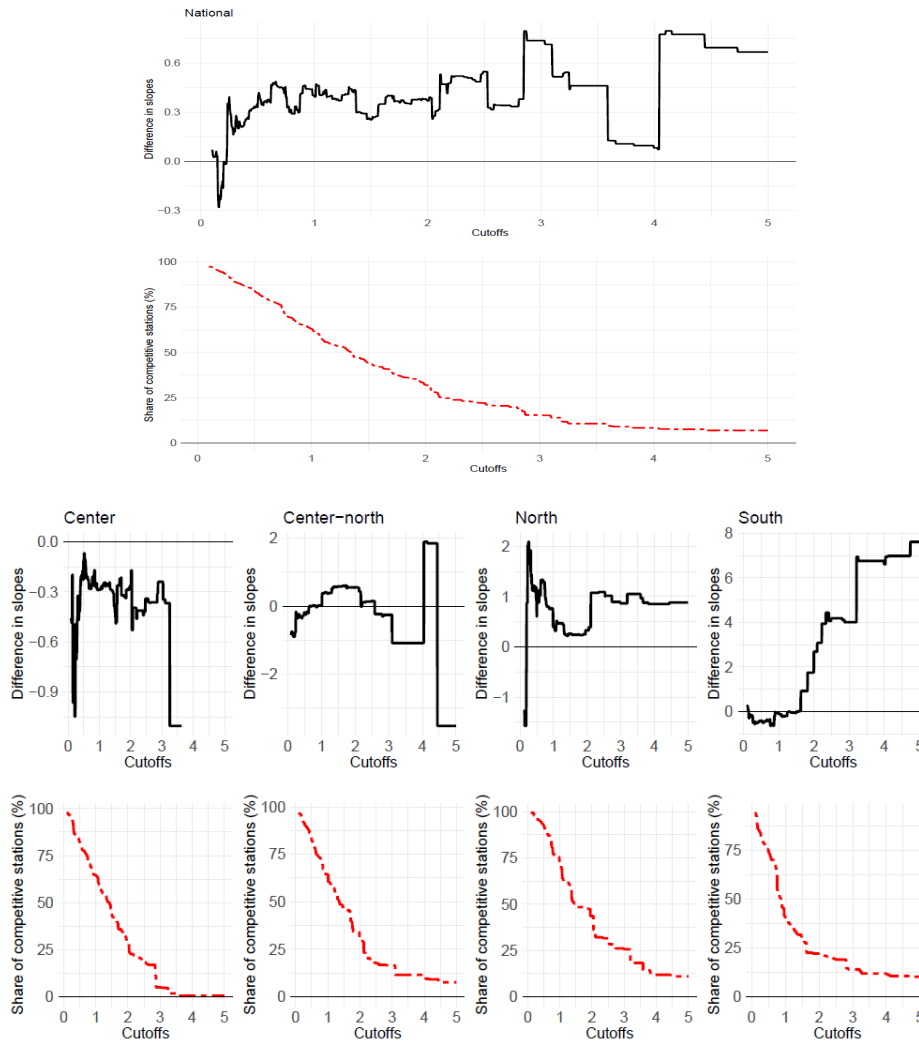
Figure D1. Robustness of classifier. Difference in regression slopes for different cutoffs of the classifier.
