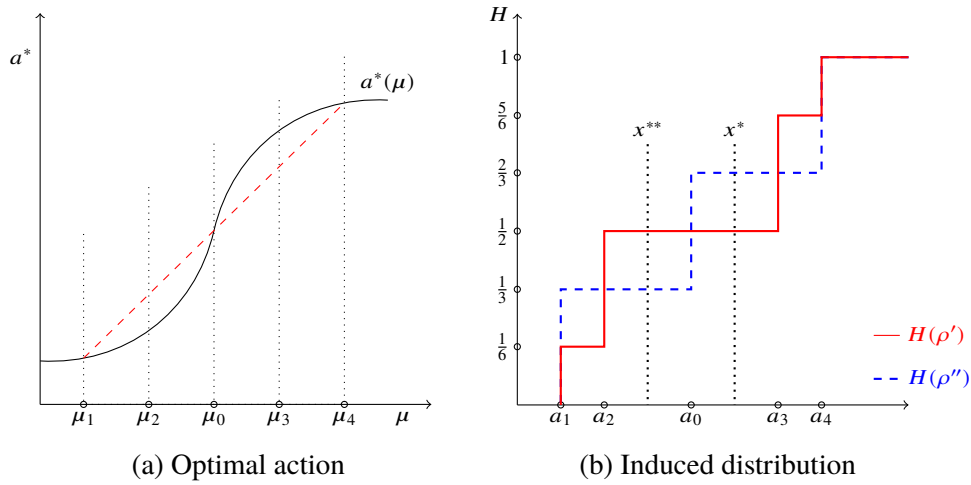
Figure 8: Non-convexity/concavity and non-responsiveness
