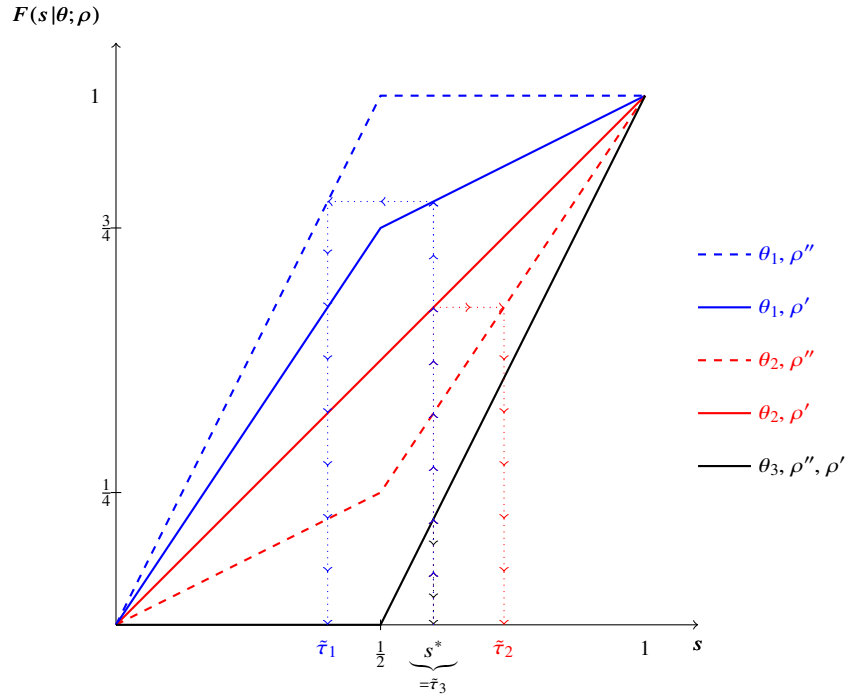
Figure 11: \rho'' \not\prec_L \rho'
