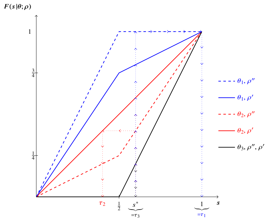
Figure 10: \rho' \not\leq_L \rho''
