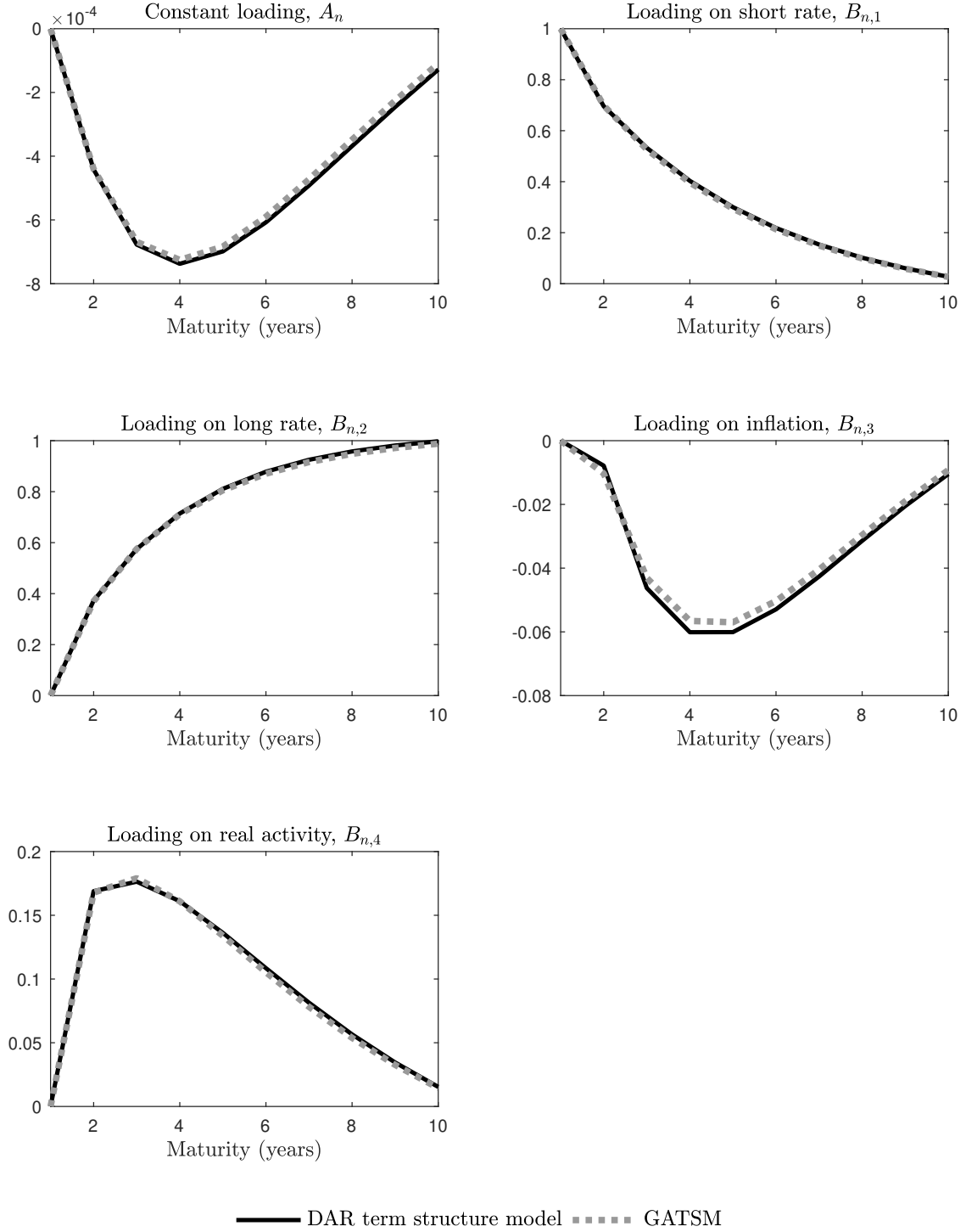
Figure 1.8: Factor Loadings
