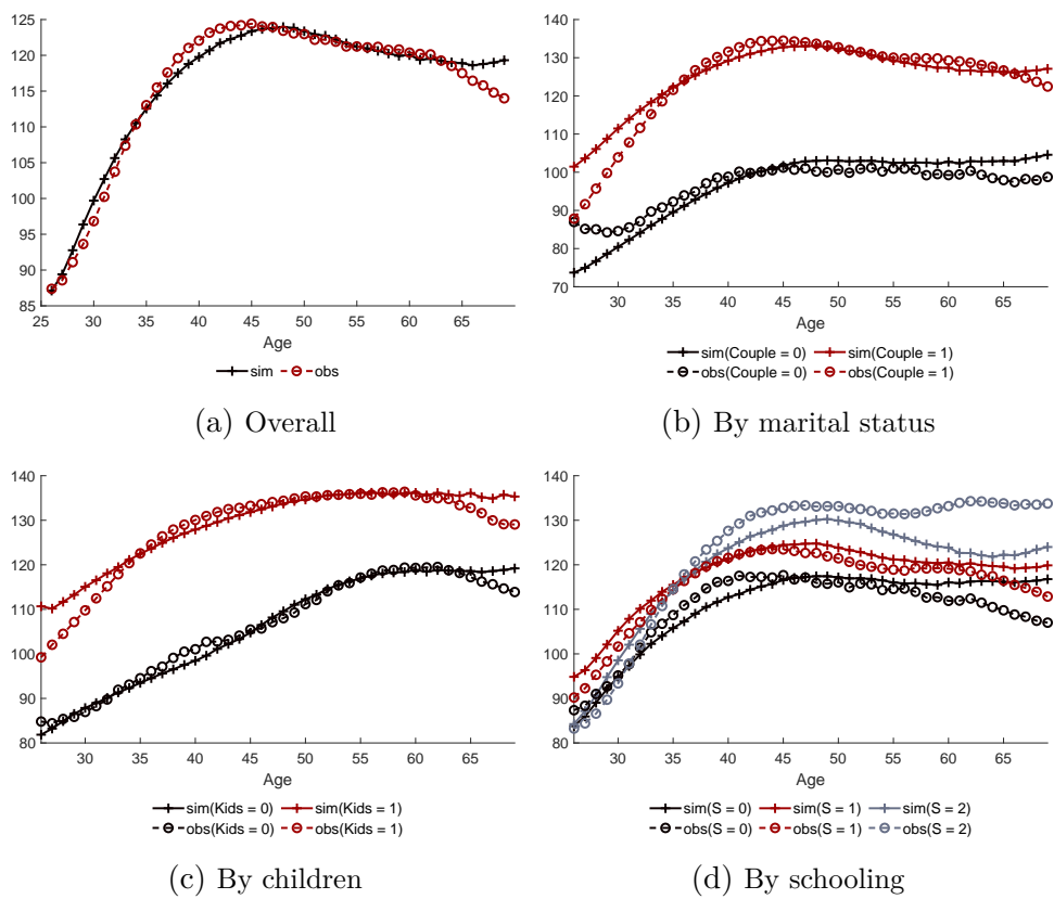
Figure 2.9: Model fit: housing size over the life cycle
