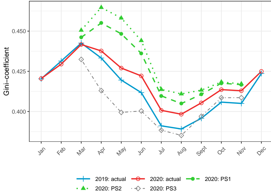
Figure 7: Inequality effect of COVID-19 policy support.
