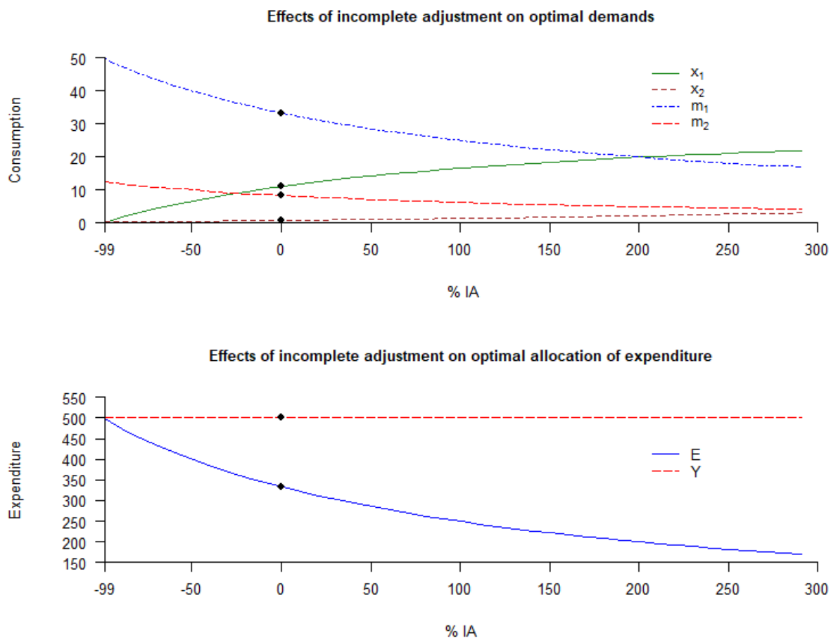
Figure 1: Optimal demands and expenditures as functions of incomplete adjustment in the parametric example. Prices are: p_1=15 , p_2=0.5 , r_1=5 and r_2=20 . Total expenditure is Y=500 . The percentage amount of incomplete adjustment (x-axis) vary between 99 and 300. Filled points are optimal demands and expenditures without incomplete adjustment.
