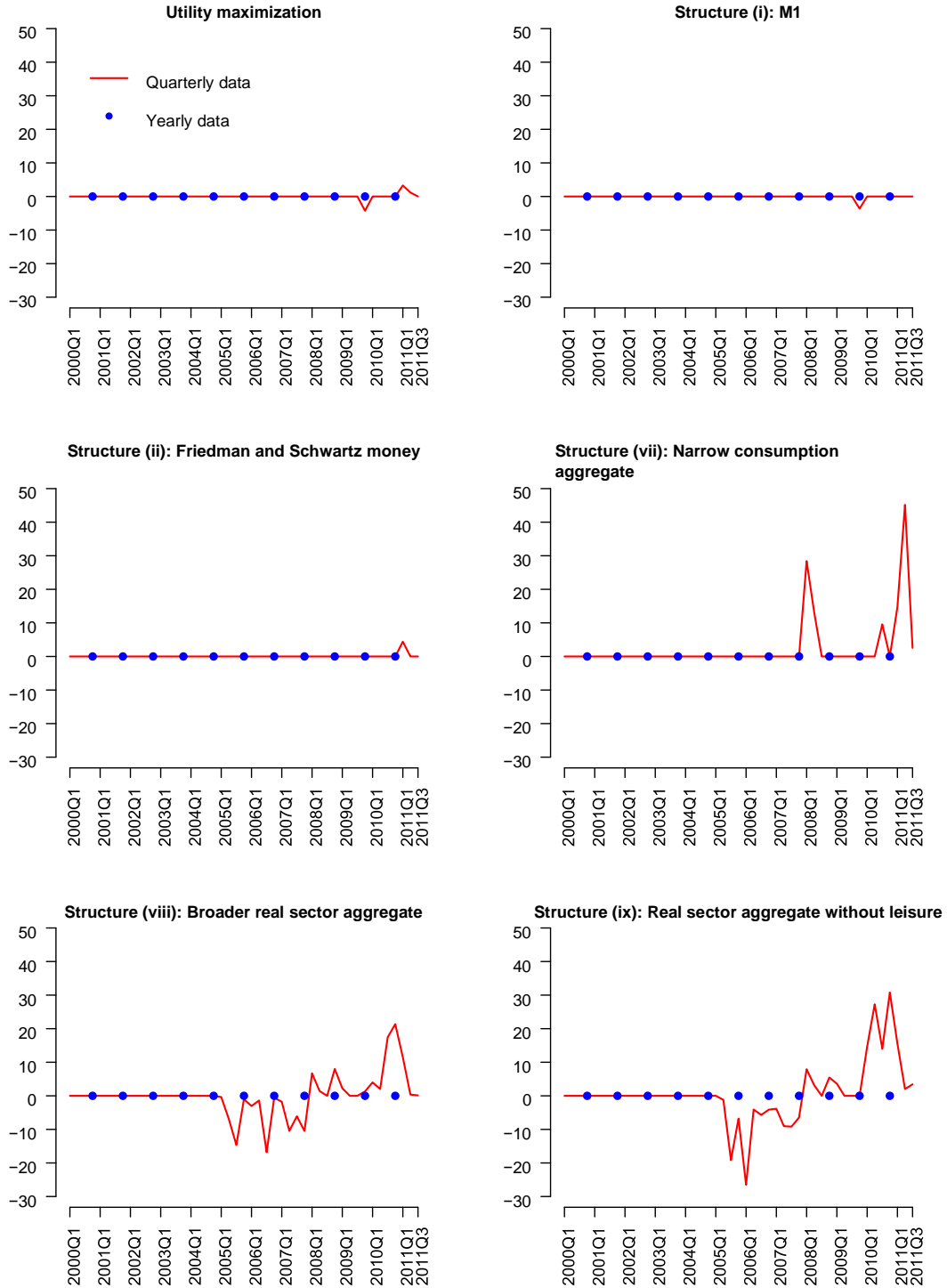
Figure 2: Minimal amount of incomplete adjustment for utility maximization and the weakly separable structures (i)-(ii) and (vii)-(ix) from Table 3.
