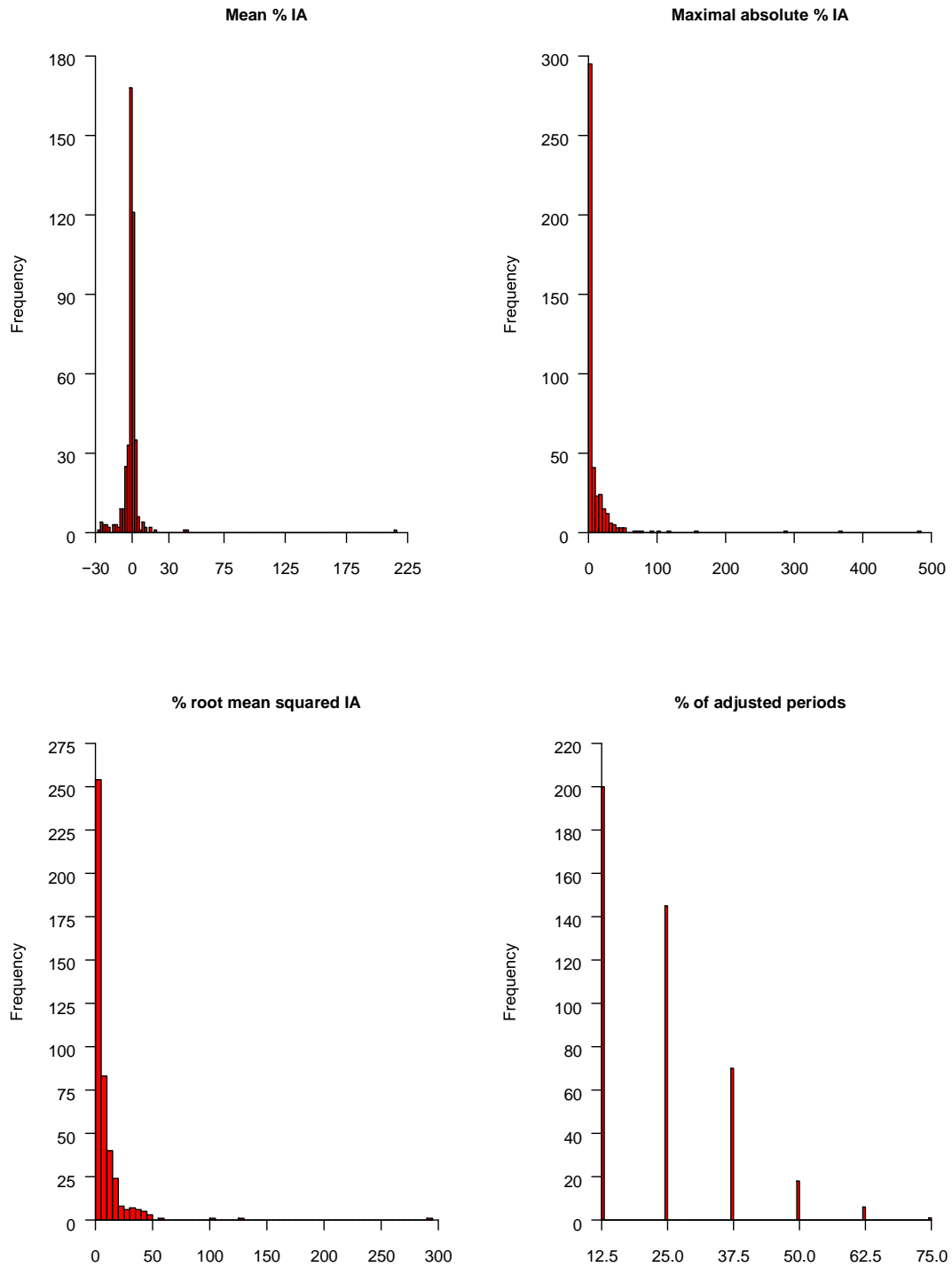
Figure 3: Histograms of the summary statistics (39)-(42) over the 440 households satisfying weak separability with incomplete adjustment in the ECPF data.
