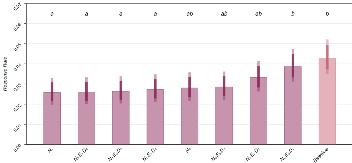
Figure 3: Study 2: Response rates separated by treatment conditions. Error bars indicate 95% and 99.5% confidence intervals (Clopper-Pearson) for proportions. Letters indicate significance groupings, that is, treatment conditions with a common letter in the group label do not significantly differ in means ( p > 0.005 ). Summary statistics are provided in Table B1; differences in response rates and the results of pairwise z -tests of proportions are provided in Table 4.
