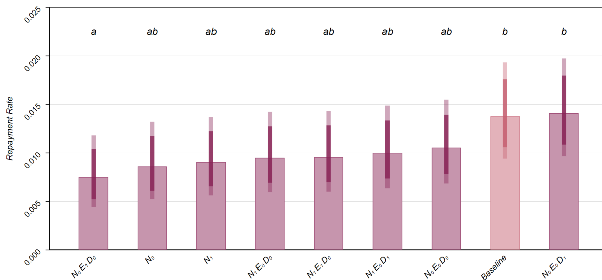
Figure B1: Study 2: Repayment rates separated by treatment conditions. Error bars indicate 95% and 99.5% confidence intervals (Clopper-Pearson) for proportions. Letters indicate significance groupings, that is, treatment conditions with a common letter in the group label do not significantly differ in means ( p > 0.005 ). Summary statistics are provided in Table B2; differences in repayment rates and the results of pairwise z -tests of proportions are provided in Table 5.
