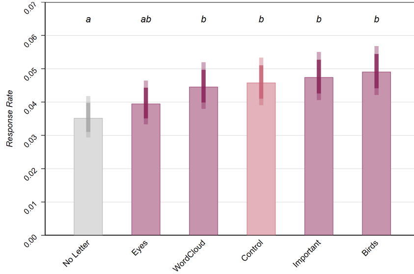
Figure 2: Study 1: Response rates separated by treatment conditions. Error bars indicate 95% and 99.5% confidence intervals (Clopper-Pearson) for proportions. Letters indicate significance groupings, that is, treatment conditions with a common letter in the group label do not significantly differ in means ( p > 0.005 ). Summary statistics are provided in Table A1; differences in response rates and the results of pairwise z -tests of proportions are provided in Table A4.
