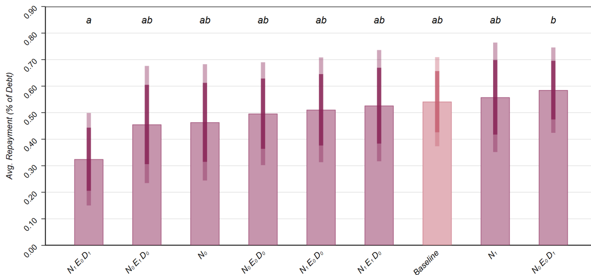
Figure B2: Study 2: Average repayments (as percentage of the outstanding debt) separated by treatment conditions. Error bars indicate 95% and 99.5% confidence intervals. Letters indicate significance groupings, that is, treatment conditions with a common letter in the group label do not significantly differ in means ( p > 0.005 ). Summary statistics are provided in Table B3; differences in repayment rates and the results of pairwise independent samples t -tests are provided in Table 6.
