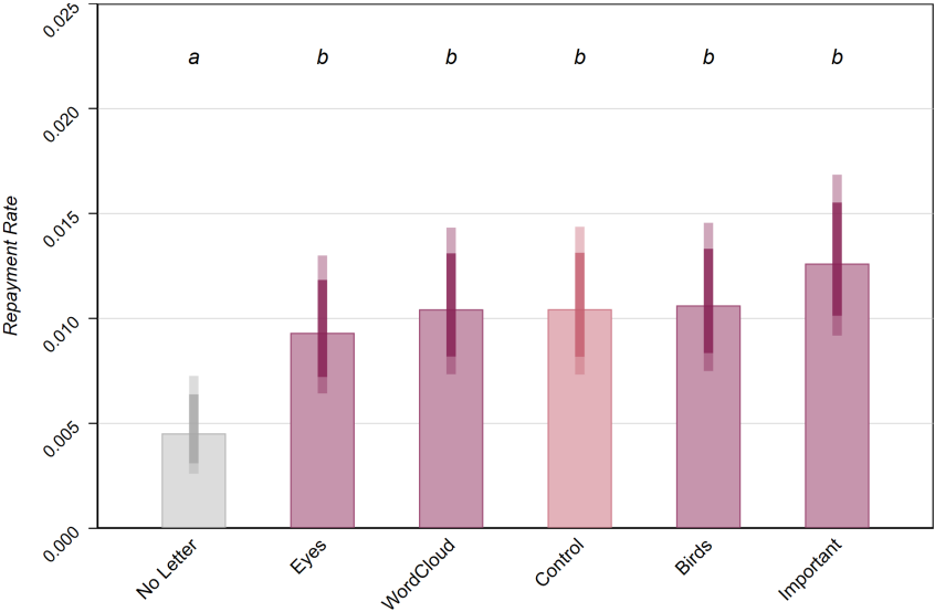
Figure A1: Study 1: Repayment rates separated by treatment conditions. Error bars indicate 95% and 99.5% confidence intervals (Clopper-Pearson) for proportions. Letters indicate significance groupings, that is, treatment conditions with a common letter in the group label do not significantly differ in means ( p > 0.005 ). Summary statistics are provided in Table A2; differences in repayment rates and the results of pairwise z -tests of proportions are provided in Table A5.
