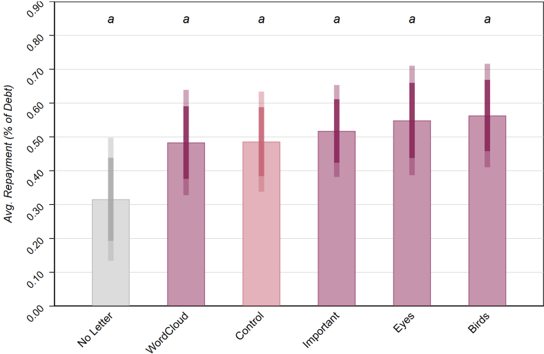
Figure A2: Study 1: Average repayments (as percentage of the outstanding debt) separated by treatment conditions. Error bars indicate 95% and 99.5% confidence intervals. Letters indicate significance groupings, that is, treatment conditions with a common letter in the group label do not significantly differ in means ( p > 0.005 ). Summary statistics are provided in Table A3; differences in repayments and the results of pairwise independent t -tests are provided in Table A6.
