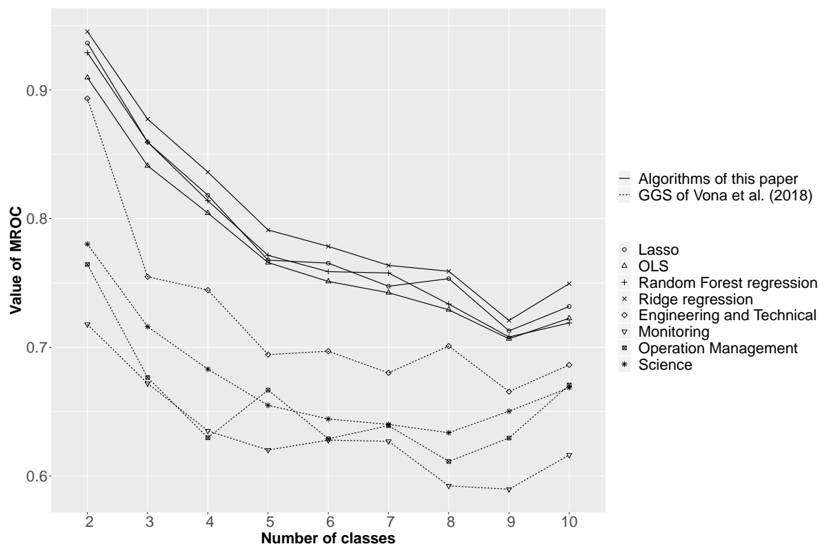
Figure 4: Multiclass Receiver Operating Characteristic Curves
