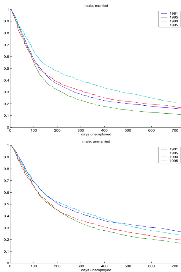
Figure 7: Kaplan-Meier-survival function estimates
