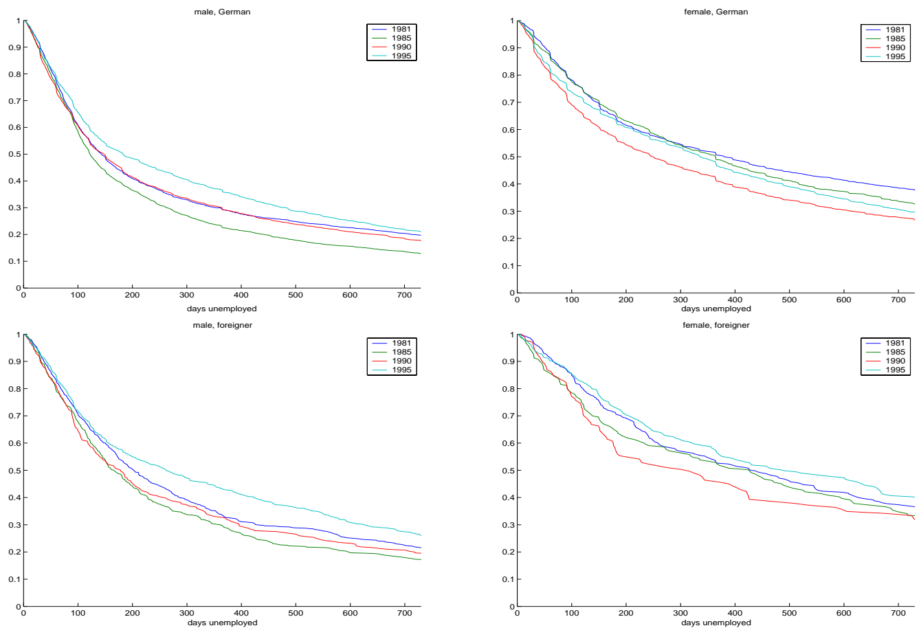
Figure 5: Kaplan-Meier-survival function estimates
