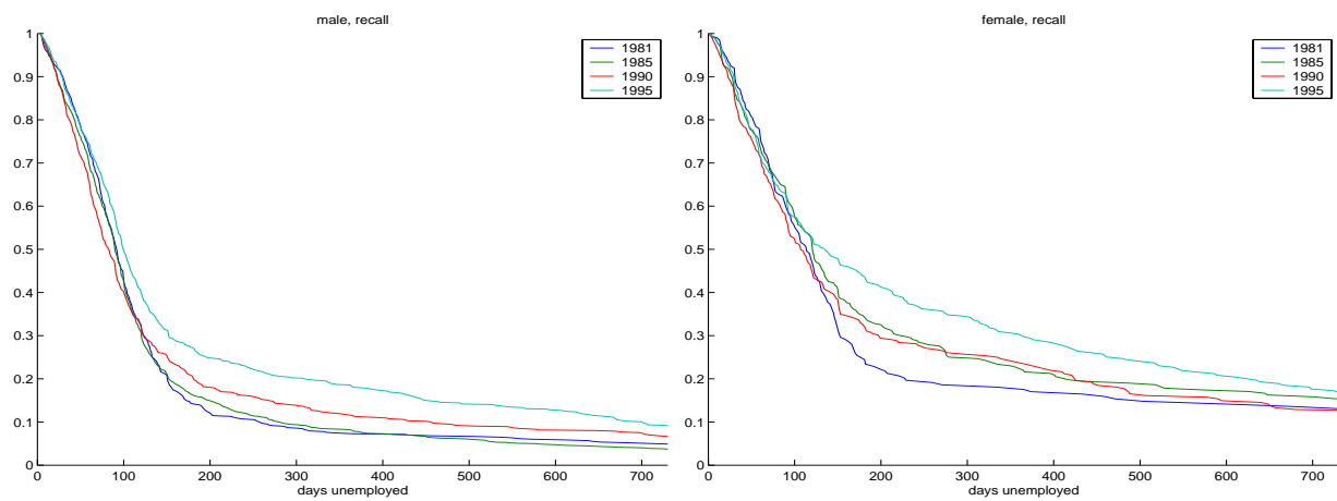
Figure 10: Kaplan-Meier-survival function estimates
