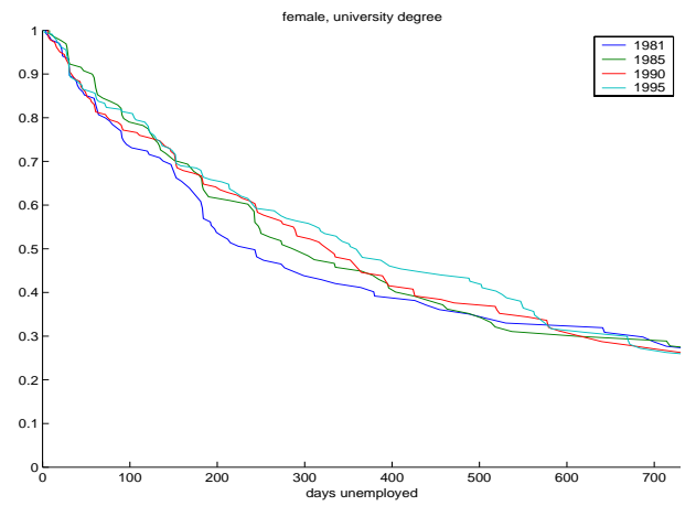
Figure 6: Kaplan-Meier-survival function estimates
