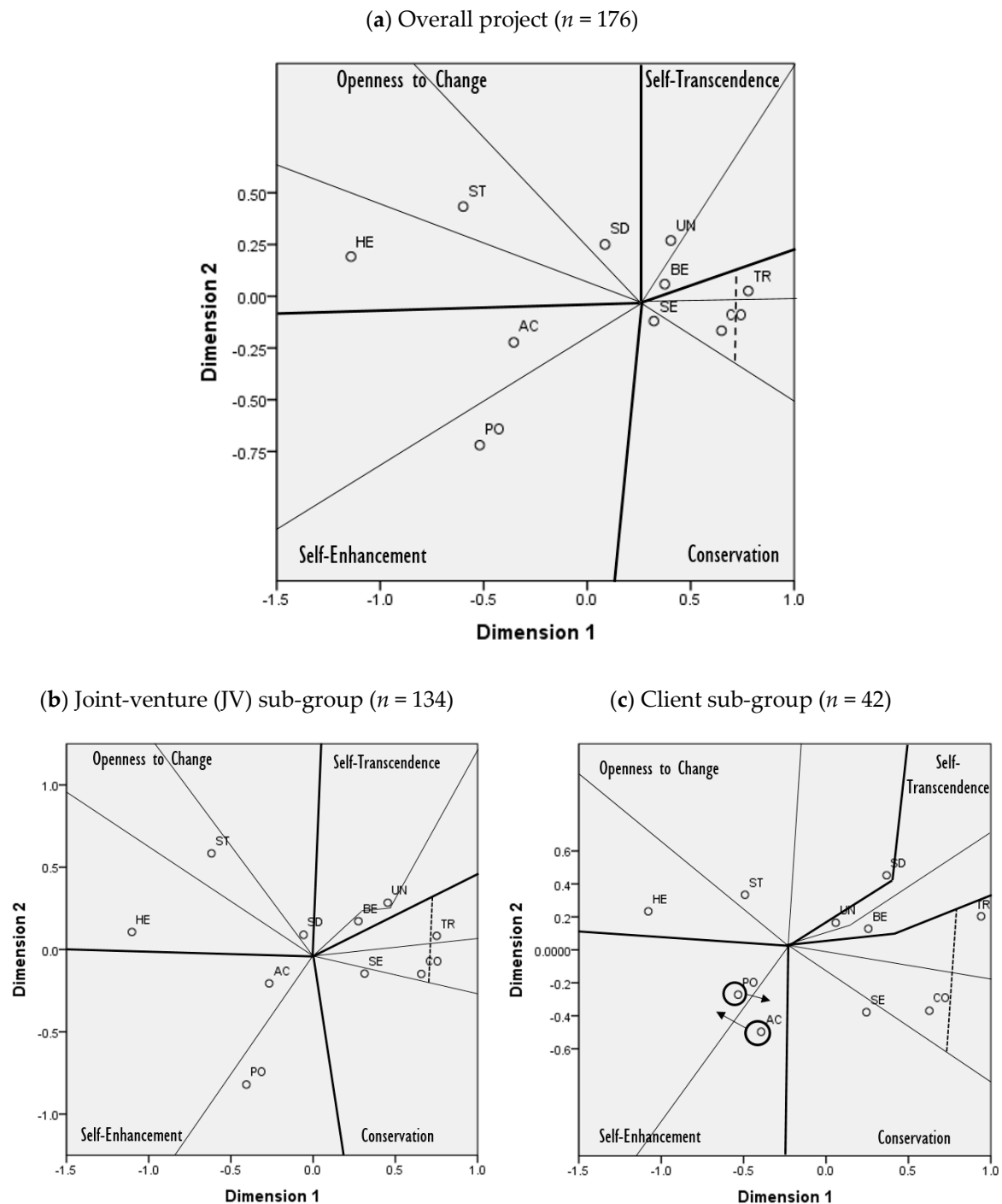
Figure 2. (a–c) Two-dimensional multidimensional scaling (MDS) of the overall project values data, including the sub-groups. Key to value categories: UN = Universalism, BE = Benevolence, TR = Tradition, CO = Conformity, SE = Security, PO = Power, AC = Achievement, HE = Hedonism, ST = Stimulation, SD = Self-Direction.
