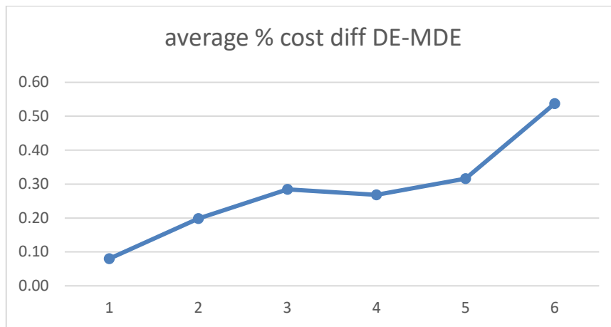
Figure 4. Average percent difference between DE and MDE. 1, 2, 3, 4, 5, and 6 represent computational times of 10, 30, 40, 60, 80, and 60 min, respectively.
