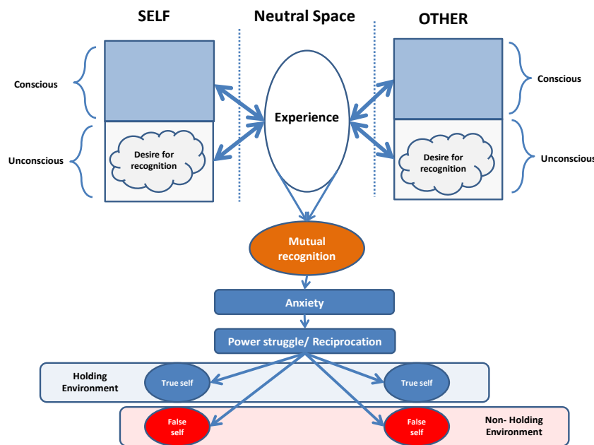
Figure 2. Winnicott’s Model.
