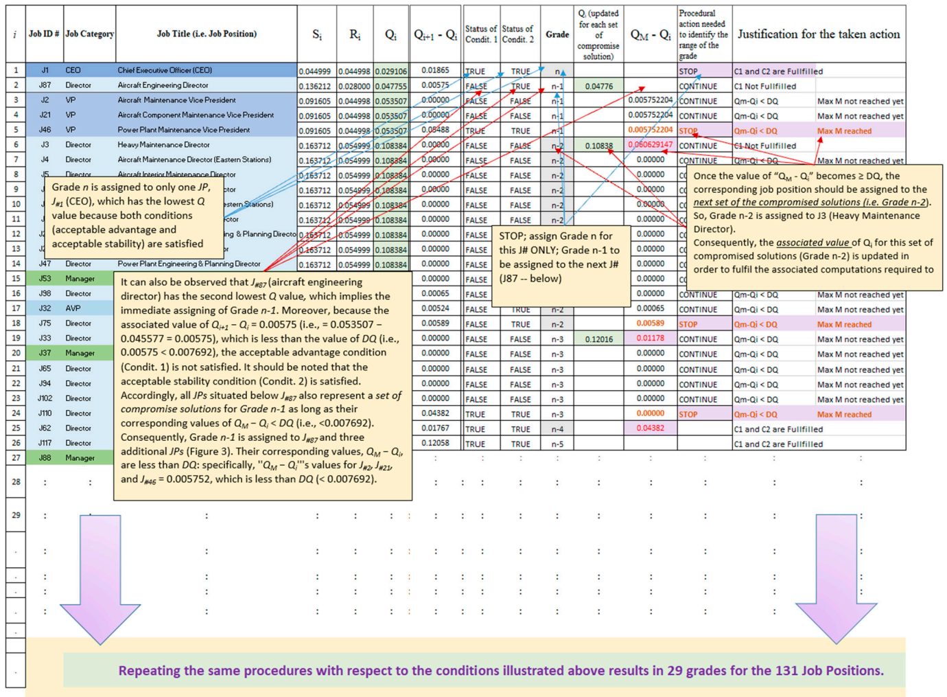
Figure 3. Grade identification using the VIKOR algorithm.
