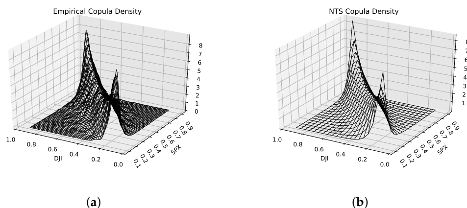
Figure 9. Density of (a) the empirical copula and (b) the NTS copula.
