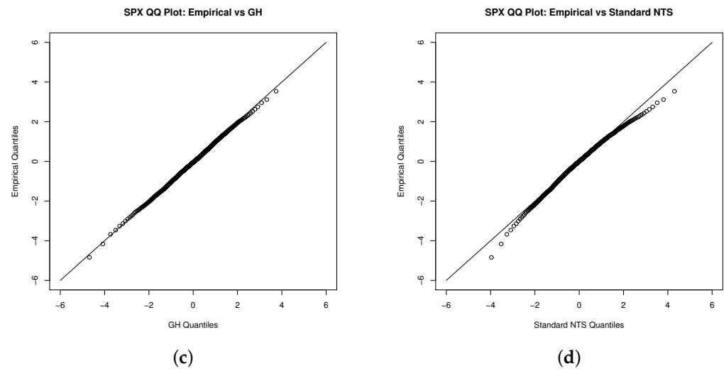
Figure 2. QQ plot for the innovations of the S&P 500 index with (a) the Student's t, (b) NIG, (c) GH, and (d) standard NTS distribution.
