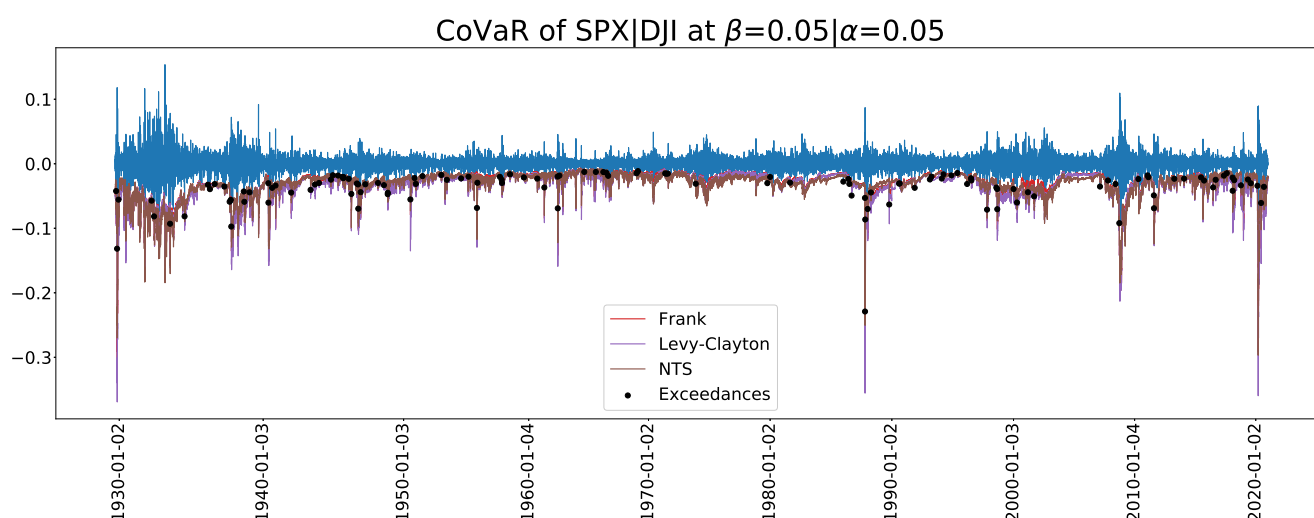
Figure 12. A CoVaR plot for \alpha = \beta = 0.05 .
