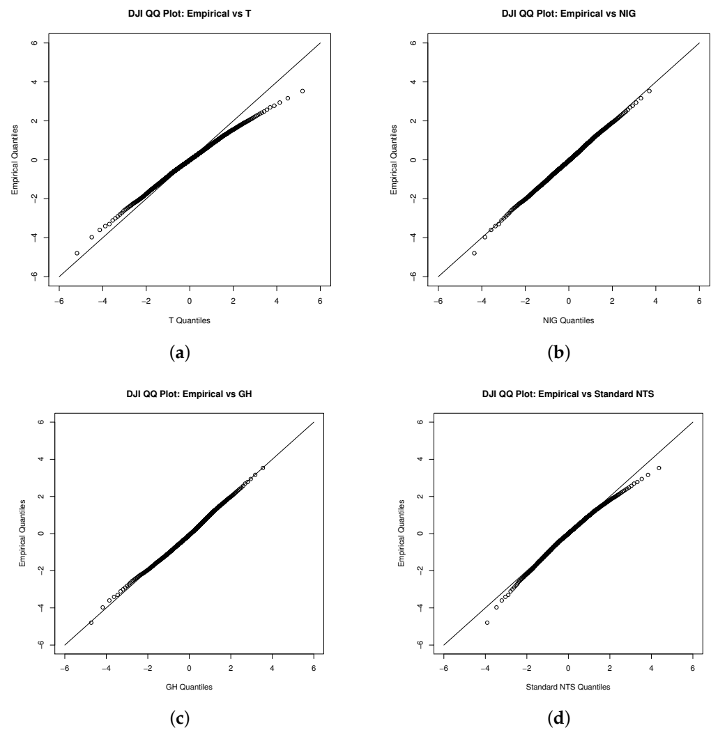
Figure 3. QQ plot for the innovations of Dow Jones index with (a) the Student's t, (b) NIG, (c) GH, and (d) standard NTS distribution.
