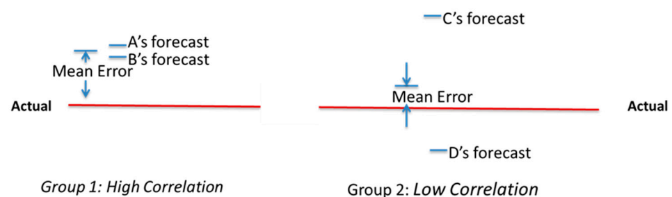
Figure 1. Individual versus group forecast accuracy—role of correlation.
