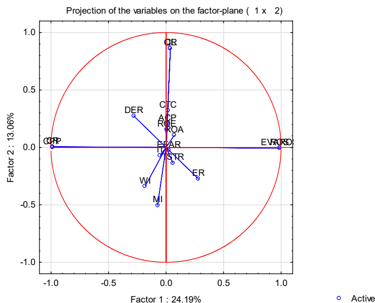
Figure 3. Projection of variables.
