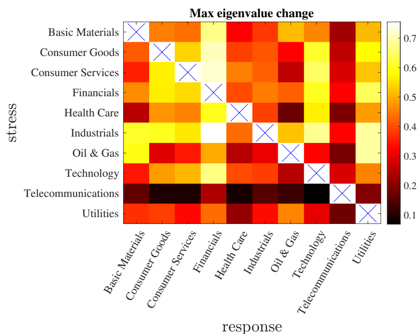
Figure A1. Change in the length of the principal axis, \Delta_{X \rightarrow Y} .
