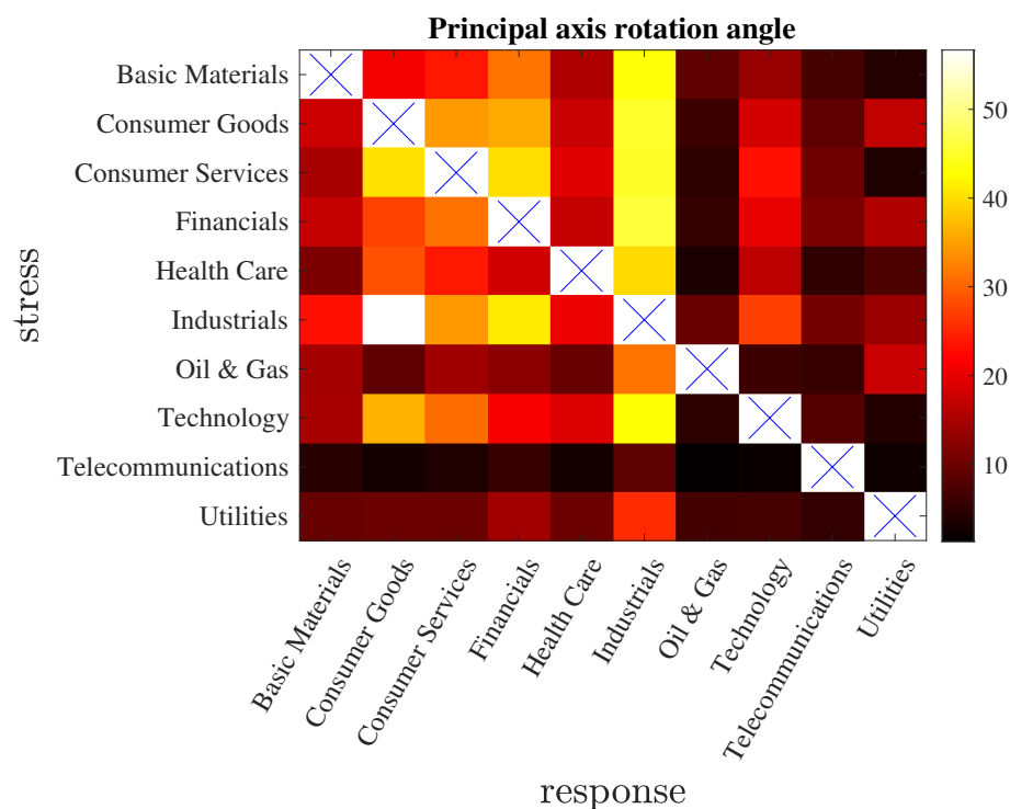
Figure 5. Angles of rotation, \Theta_{X \rightarrow Y} , of the principal axes as consequence of conditioning (degrees). The rows are the conditioning variables and the columns the conditioned ones.
