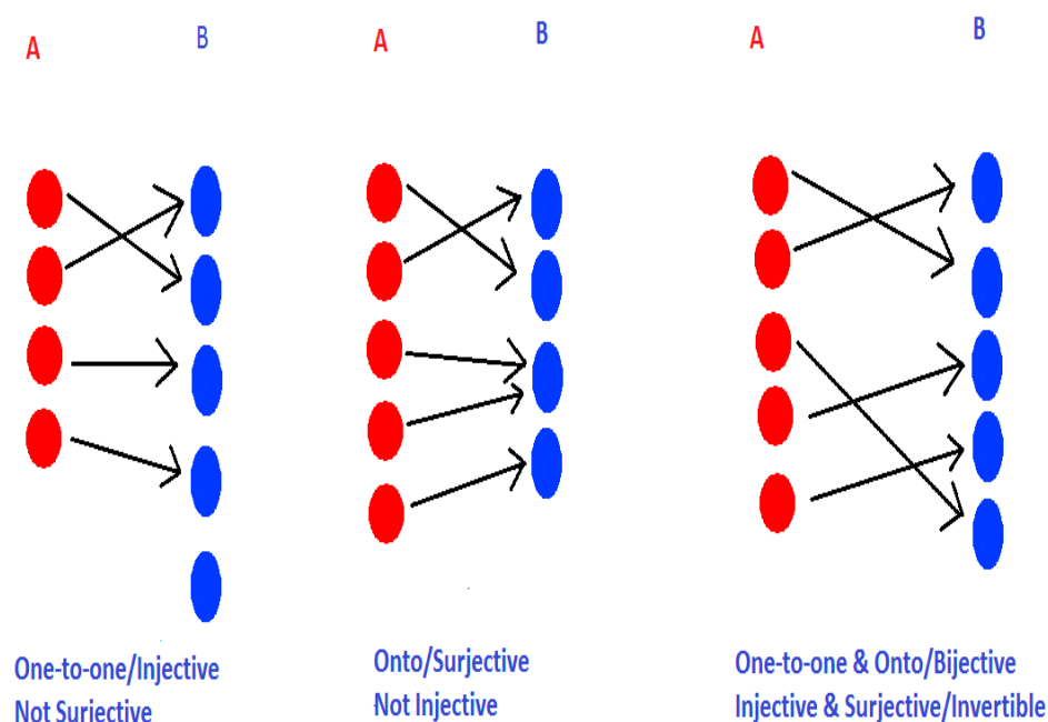
Figure A1. One-to-one, onto and invertible functions from set A to set B.
