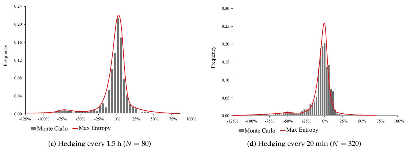
Figure 1. Distribution of hedging error of a one-month European call option under the Weighted Gamma, obtained using Monte Carlo simulation and computing Max Entropy estimation.
