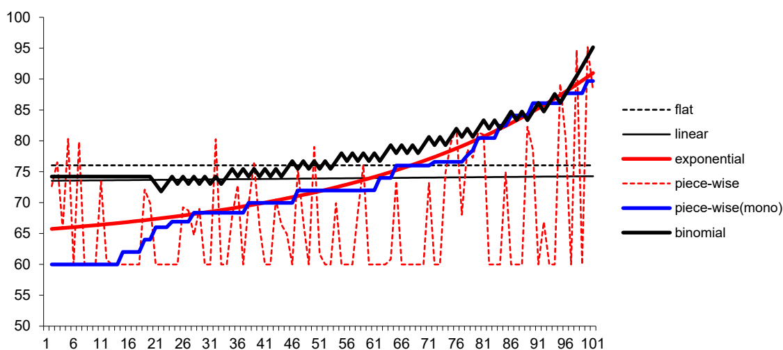
Figure 3. Various exercise boundaries.
