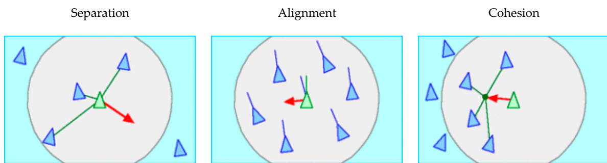
Figure 1. Three major parameters in a swarm. Sources: https://en.wikipedia.org/wiki/Boids .
