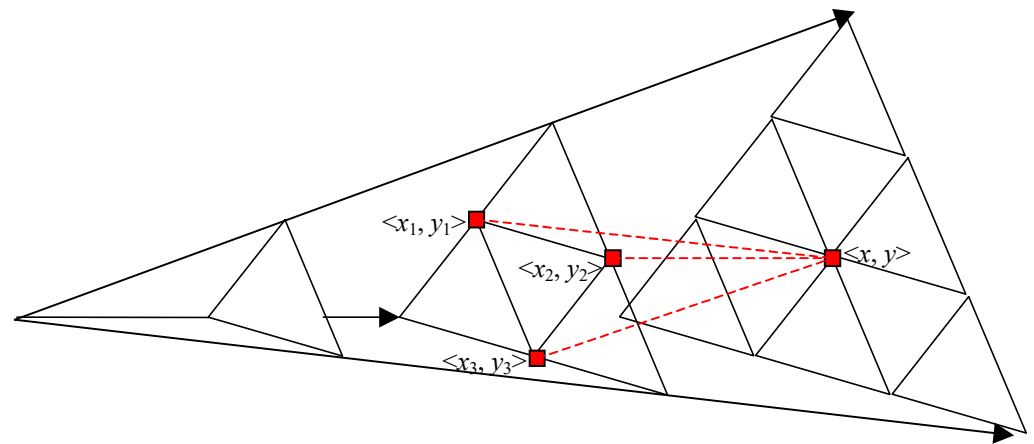
Figure A1. A two-asset Chen–Chung–Yang Model.
