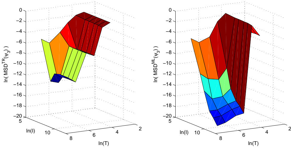
Figure 2: MSD^{TR} (left) and MSD^{ML} (right) for \psi_3 for one specimen data series
