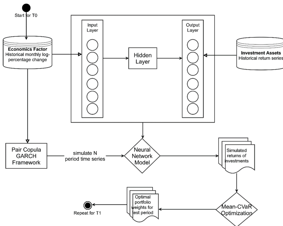
Figure 3. Process workflow diagram of Economic Factor-Based Predictive Model (EFPM).
