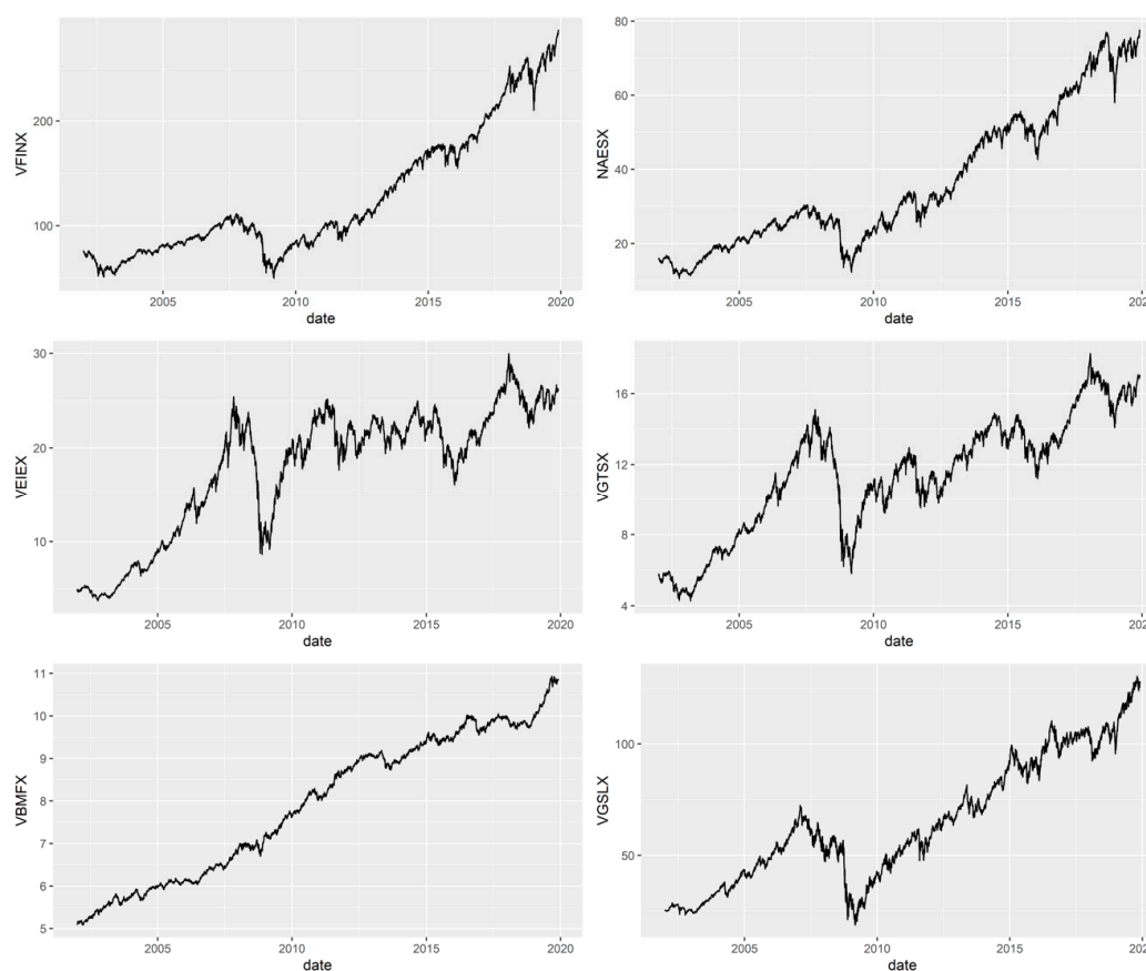
Figure 4. Time series of six index funds' prices between January 2002 and November 2019.
