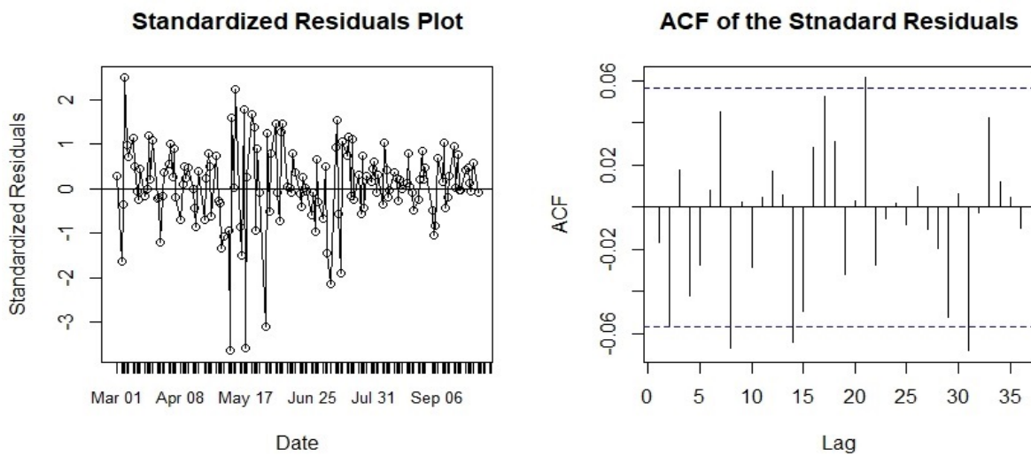
Figure 7. ARIMA(0,2,1) model residual analysis.
