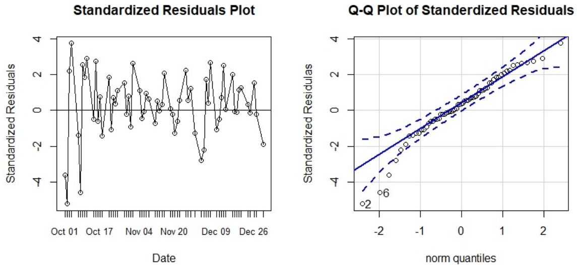
Figure 9. GBM model diagnostics.
