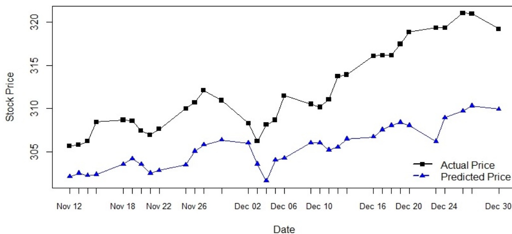
Figure 10. ANN(7-15-1) prediction.
