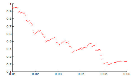
(b) IBOVESPA extremal index.
