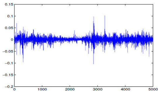
(a) PSI20 return index.
