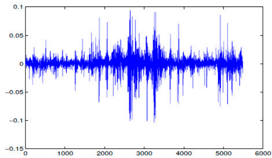
(a) IBOVESPA return index
