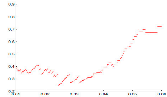
(b) IBOVESPA extremal index.
