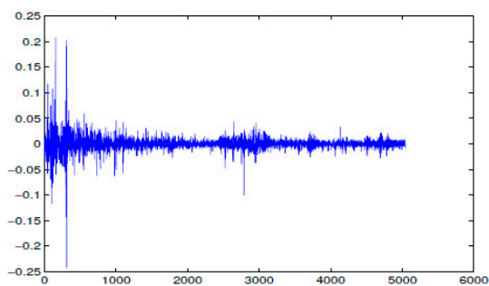
(c) MICEX return index.
