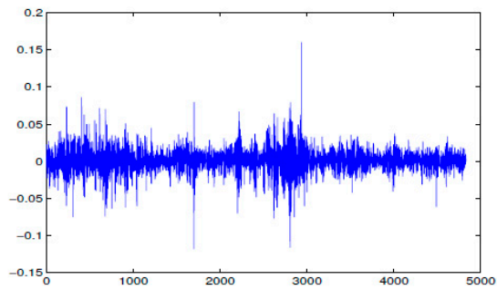
(c) TASI return index.
