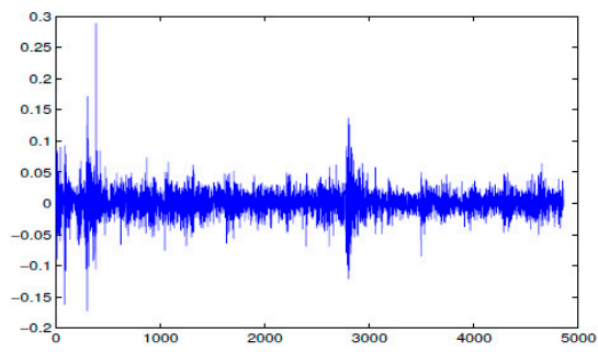
(a) IBOVESPA return index
