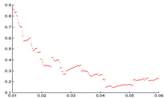
(b) PSI20 extremal index.
