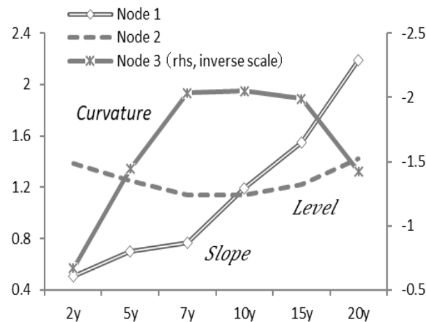
Figure 7. Coefficients of the linear function output from the hidden layer (for three nodes).
